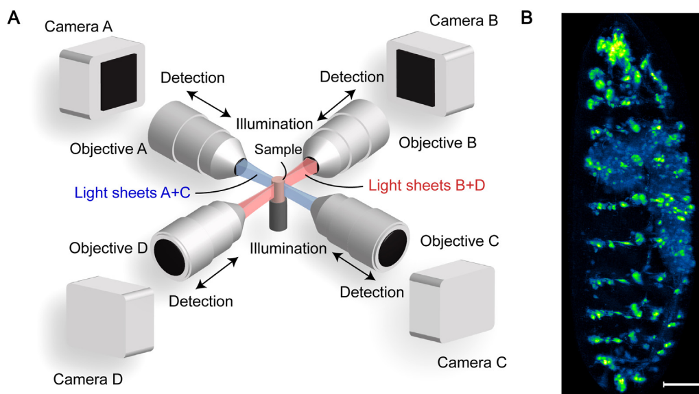
Fig. 1. Gaussian Light Sheet Imaging. (A) IsoView microscopy facilitates imaging of large biological specimens with high spatio-temporal resolution using light-sheet illumination and fluorescence detection along four orthogonal directions simultaneously. (B) Maximum-intensity projections of multiview deconvolved IsoView image data of a stage 17 Drosophila embryo expressing GCaMP6s throughout the nervous system. A false-color look-up table is used for better visibility of high-dynamic-range images. Figure adapted from Chhetri et al., 2015; scale bar is 50 \mu\text{m} .
